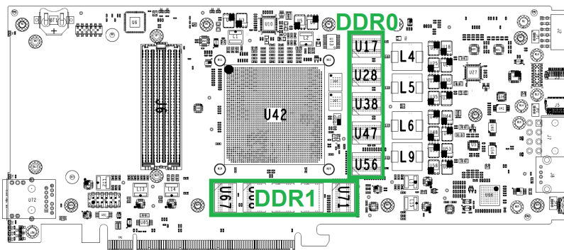
Figure 10 : DDR4 bank locations by index
