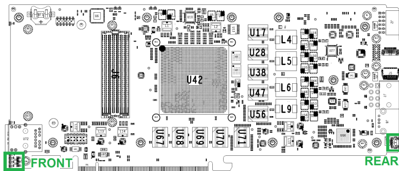
Figure 13 : USB Location
